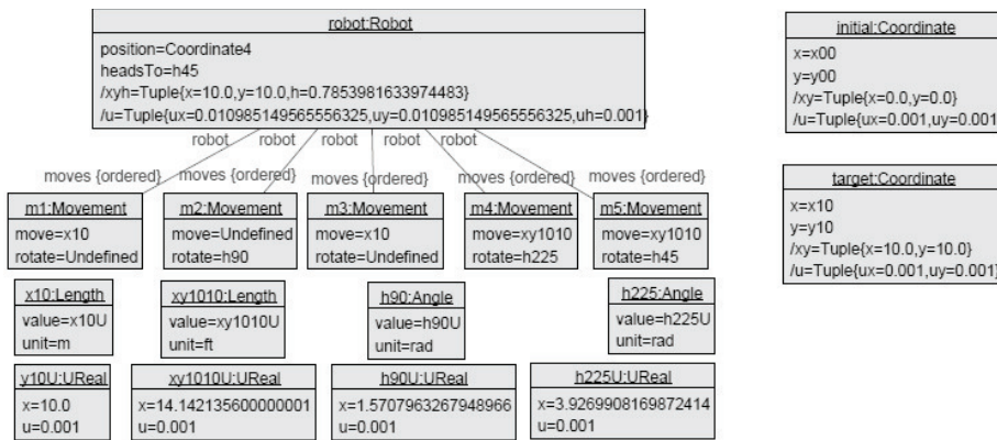
Figure 4: Object diagram for the Moving Robot example, after execution.
