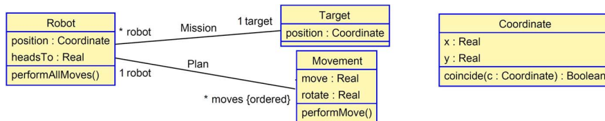
Figure 2: Initial Class diagram for the Moving Robot example, using plain UML.
