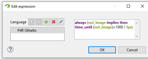
Fig. 5. P4R Othello as selected language and the defined expression
