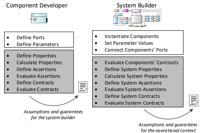
Fig. 1. Extended functionalities (in gray) provided by the P4R Assertions
