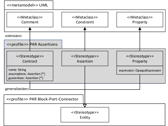
Fig. 2. P4R Assertions profile
