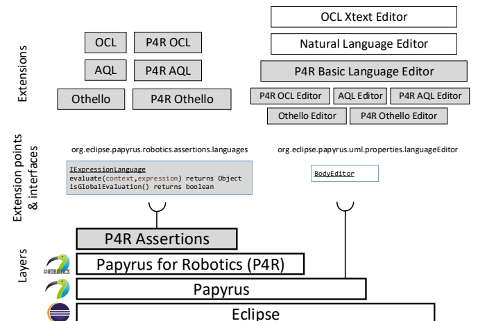
Fig. 3. Layers and languages extensibility
