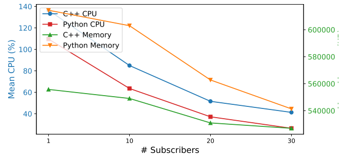
Figure 7: CPU and memory scalability of Node 3.
